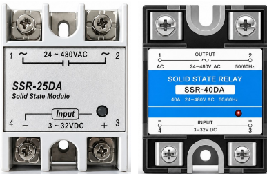
STANDARD 1-PHASE SSR
